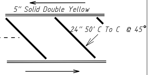
Detail D
