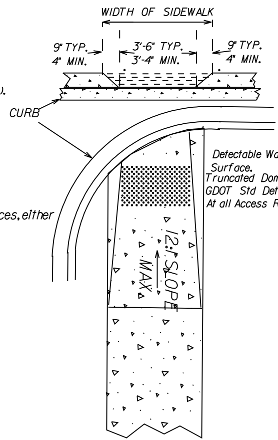
SIDEWALK RAMP DETAIL
